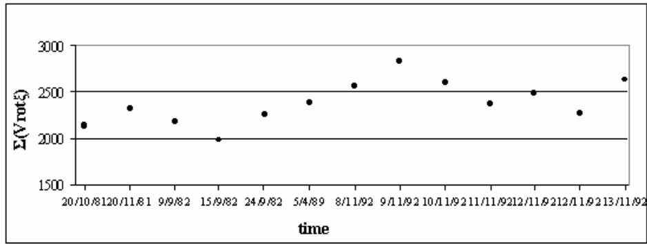
Diagram 5: (Data from table 1) Variation of \Sigma(V_{rot}\xi) as a function of the date. \Sigma(V_{rot}\xi) is an expression of the overall absorbed energy in the regions where the satellite components of both of the doublets lines are created.
