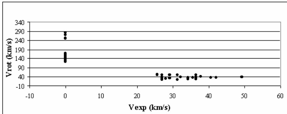
Diagram 1: (Data from table 1) Rotation velocities ( V_{rot} ) as a function of the expansion velocities ( V_{exp} ). One can see that two levels of V_{exp} are present, one of 0 km/s and another between 26 to 50 km/s. When V_{exp}=0 , two levels of V_{rot} appear, one of about 150 km/s and another of about 270 km/s. The three levels of V_{rot} appear clearly in diagram 3. When V_{exp} lies between 26 and 50 km/s, V_{rot} is about 40 km/s.
