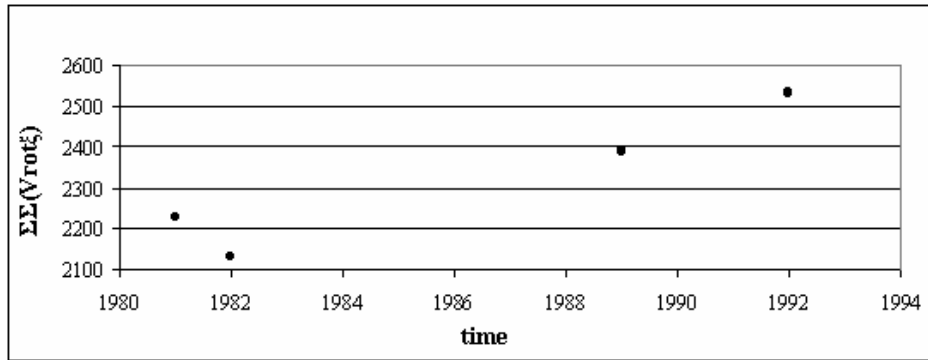
Diagram 11: (Data from table 2) Variation of \Sigma\Sigma(V_{rot}\xi) as a function of the date. From 1981 to 1992, we observe an important increase of the expression of the overall absorbed energy in the region where the SiIV resonance lines are created.
