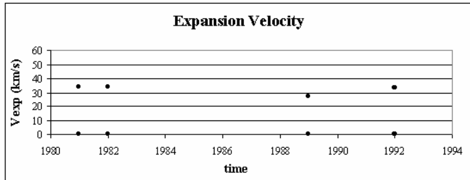
Diagram 7: (Data from table 2) Variation of the two levels of the mean apparent V_{exp} as a function of the date. The two levels of V_{exp} remain almost constant around the values of 0 and 34 km/s.
